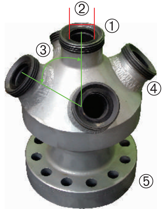
"Goat Head" Style Frac Head
