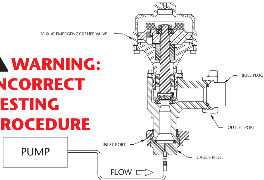
FIGURE 7. EXAMPLE OF IMPROPER TESTING SET UP OF EMERGENCY RELIEF VALVE
